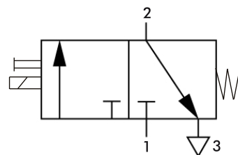
Schema idraulico Hydraulic scheme
