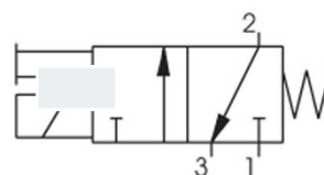
Schema idraulico Hydraulic scheme
